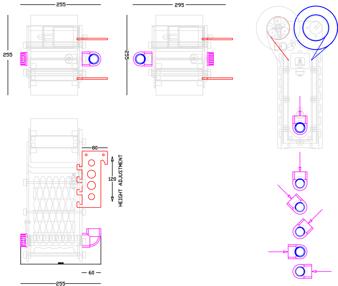
STANDARD BRACKET
